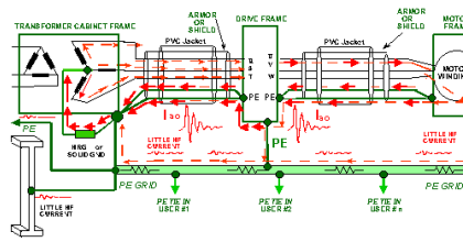
Fig. 20 CM high frequency noise path taken for recommended IGBT drive installation with shielded output wires with insulated
