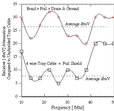
Fig. 23 Relative high frequency shielding effectiveness of tray cable compared to Type TC plus foil vs. Focus cable braid/foil/ground wire system.
