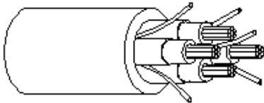
Fig. 2 Vinyl Nylon Tray Cable using 4 PVC-Nylon THHN conductors, fillers and an overall PVC outer jacket.
