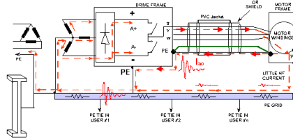
Fig. 19 CM high frequency noise path taken for preferred IGBT drive installation with shielded output wires plus insulated ground in a PVC jacket. Shield and ground wires are bonded at both drive and motor grounds.
