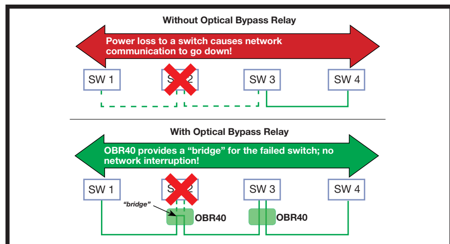
Example of Optical Bypass Relay without and with OBR40 installed
