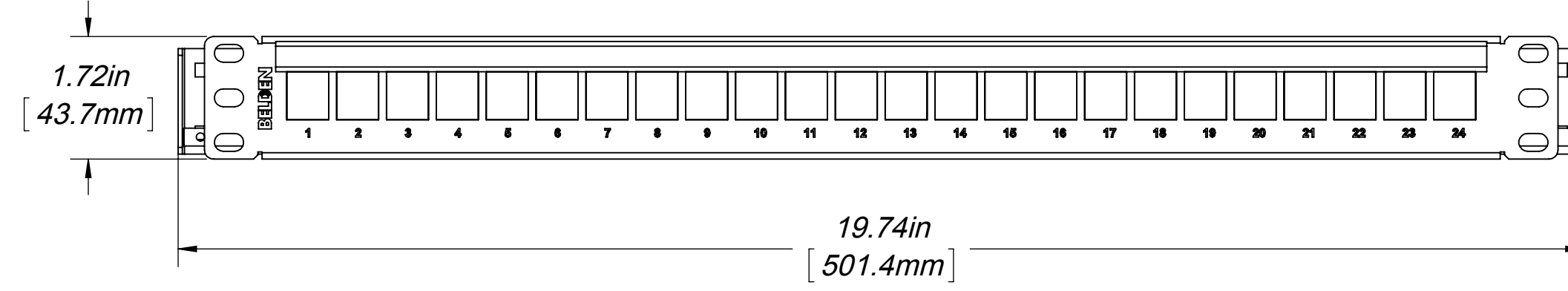
AX103114 EMPTY VARIANT SHOWN FOR REFERENCE DIMENSIONS
